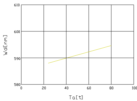
Fig.5-Dominant Wavelength(@250mA) vs. Ambient Temperature
