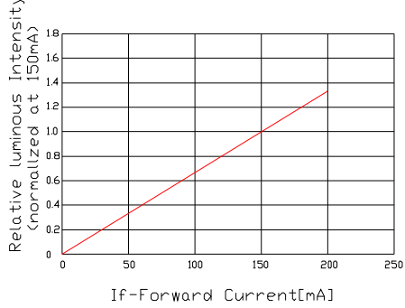
Fig.1-Relative luminous Intensity vs. Forward Current
