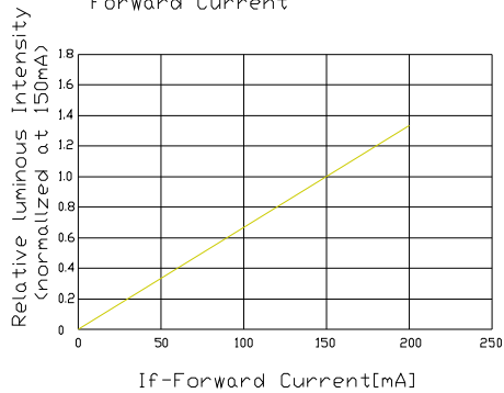
Fig.1-Relative luminous Intensity vs. Forward Current
