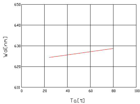
Fig.5-Dominant Wavelength(@150mA) vs. Ambient Temperature
