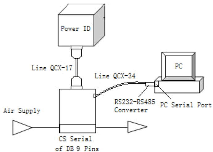
Figure 2-11 CS Product and Illustration of Connecting Power D08-1D/1F
