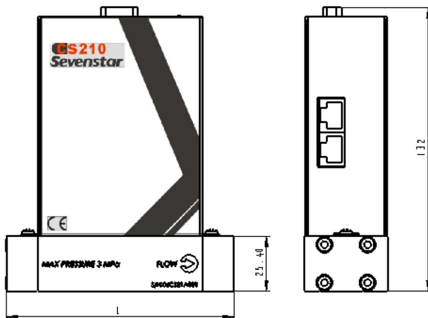
Figure 2-2a Product with A-seal dimensions
