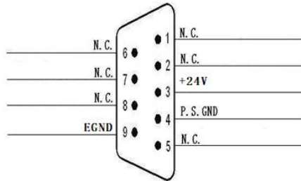
Figure 2-8 9 pin male D-sub connector
