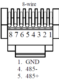
Figure 2-9 RS485 connector
