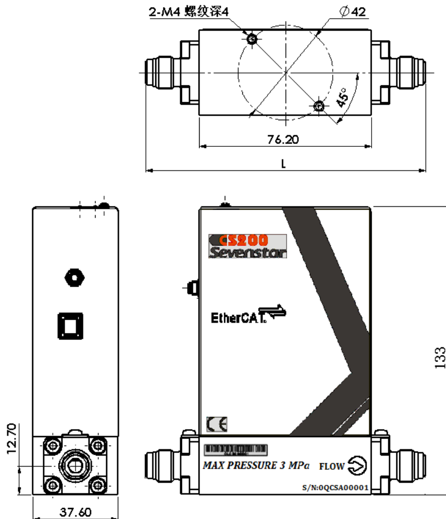
Figure 2-4 CS210-C(EtherCAT) Product dimensions
