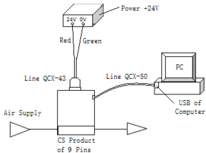
Figure 2-12 CS Product and Illustration of Connecting Power
