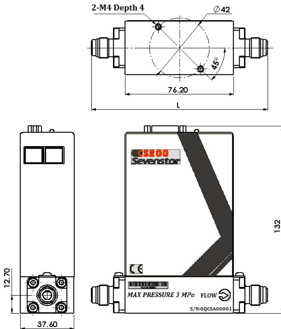
Figure 2-2 CS210-C(RS-485) Product dimensions
