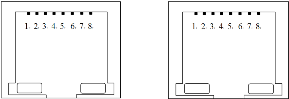
1、TX+ 2、TX- 3、RX+ 6、RX- Figure 2-10 EtherCAT connector of RJ45
