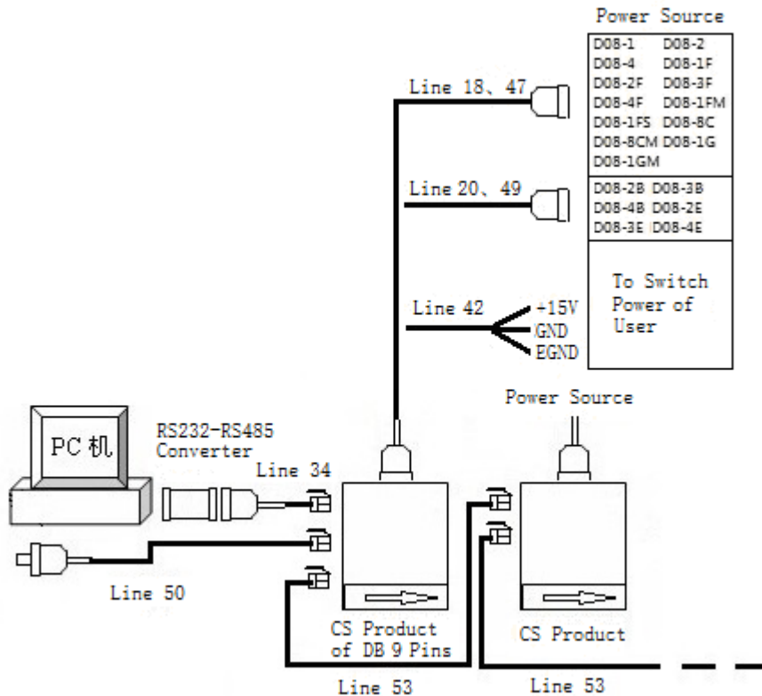
Figure 2-13 Illustration of Connecting CS Product
