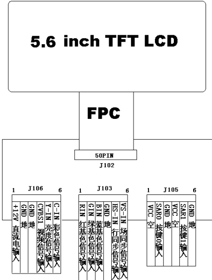
A/D board:GDN-D567AT
