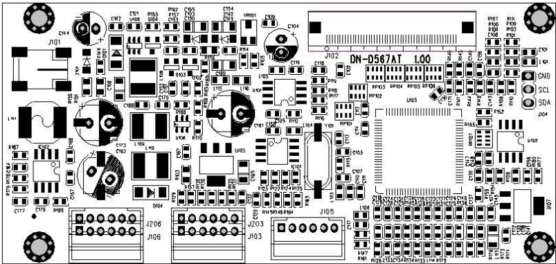
A/D board:GDN-D567AT
