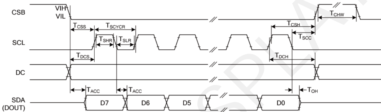
Figure: 4-wire Serial Interface Characteristics (Read mode)
