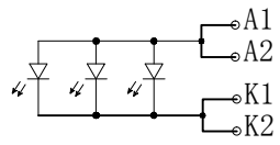
CIRCUIT DIAGRAM(LED 1*3=3 DIES)
