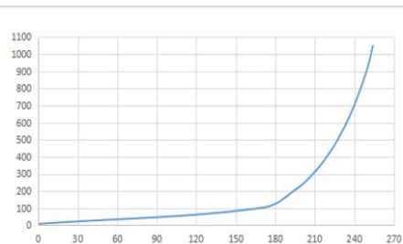
DALI Dimming Curve (logarithmic)
