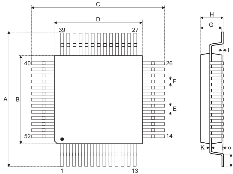
52-pin QFP (14mm×14mm) Outline Dimensions
