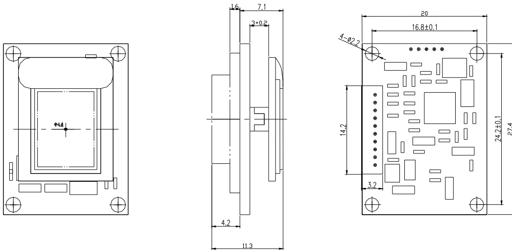
Installation diagram with SVGA060 OLED
